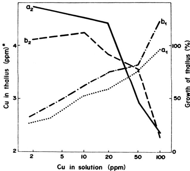
Figure 38 Copper accumulation and relative growth of thallus of soil micromycetes as a function of the metal concentration in nutrient solution. (a 1 ) Penicillium sp. from soil polluted with Cu—accumulation of metal, (a 2 ) growth of Penicillium sp., relative to control, (b 1 ) Penicillium chrysogenum from unpolluted mineral soil—accumulation of metal, (b 2 ) growth of Penicillium chrysogenum , relative to control. 1195 *Values given in powers of ten.
