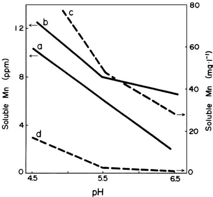
Figure 96 Solubility of soil Mn at different pH values. (a) In 0.01 M CaCl 2 from bulk soil; (b) in 0.01 M CaCl 2 from rhizosphere soil; (c) in 0.01 M citrate solution; (d) in root exudates, after 72 hr. 270
