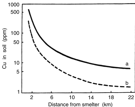
Figure 35 Smoothed patterns for Cu concentrations in soils as a function of downwind distance from a Cu smelter (mean values of 3 years); (a), total content; (b), soluble content. 380
