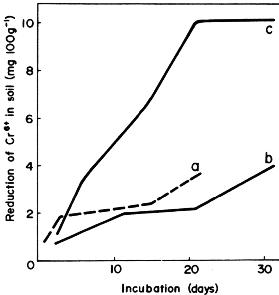
Figure 86 Reduction of Cr 6+ by soil (pH 6.7) during the incubation. (a) Aerobic; (b) anaerobic; (c) anaerobic with added dry alfalfa material. 82
