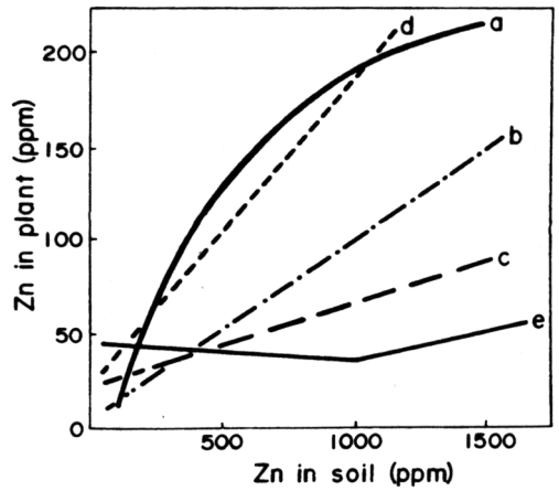
Figure 46 Zn uptake by plants from soil contaminated by this metal. (a) Pasture herbage, (b) wheat straw, (c) wheat grains, (d) potato stalks, (e) potato tubers. 176,783
